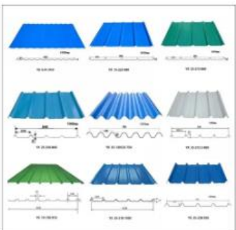
Ppgi Roofing Sheet
